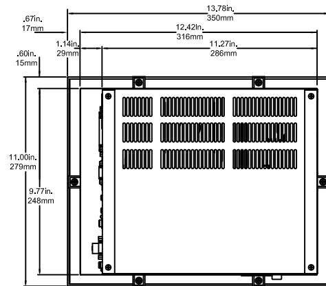
HPC HPX 10" Back View
