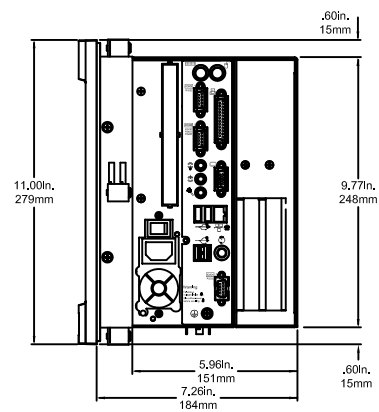
10" Daytona Right View with PCI Expansion
