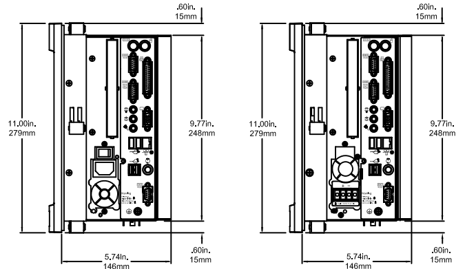
HPC HPX 10" Right View AC and DC
