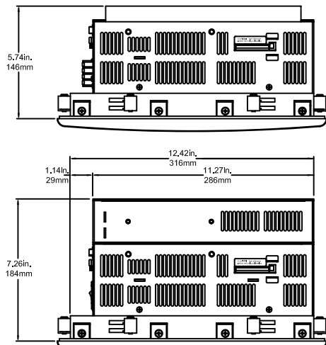
HPC HPX 10" Bottom View Base and PCI Expansion
