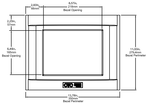
HPC HPX 10" Front View
