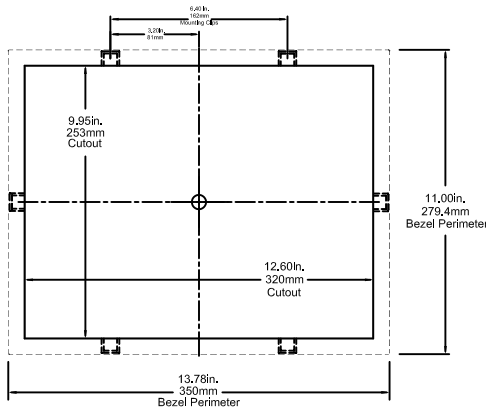
HPC HPX 10" Mounting
