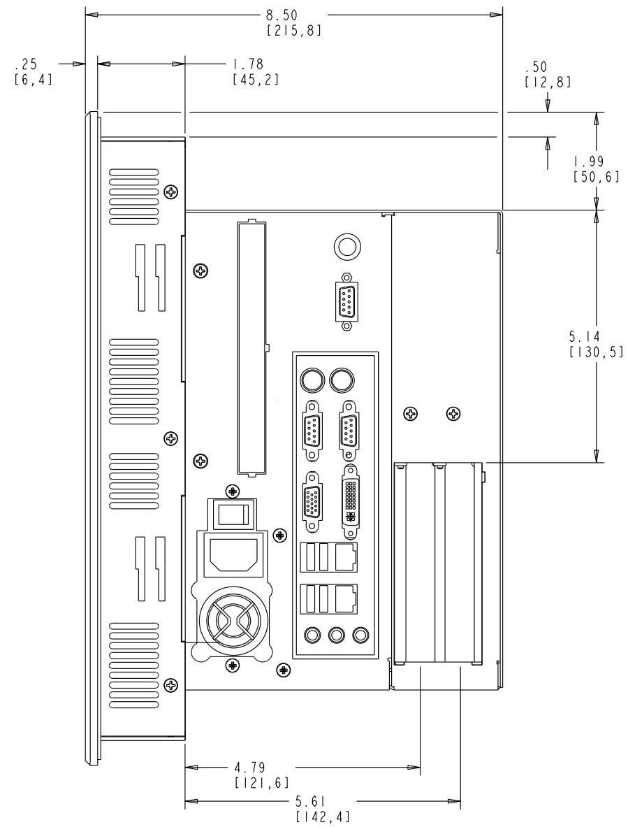
IPX/IPC EXPANSION CHASSIS SIDE VIEW
