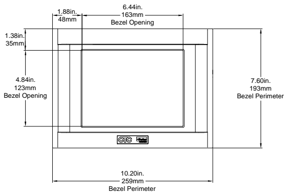
PA08S & PA08T Front View
