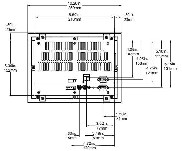
PA08S & PA08T Back View
