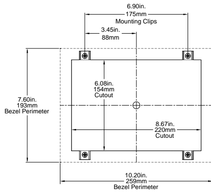
PA08S & PA08T Mounting
