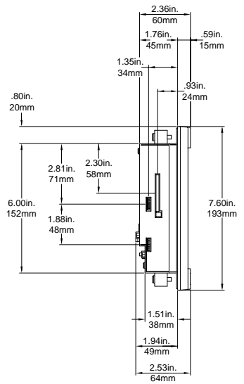
PA08S & PA08T Left Side View
