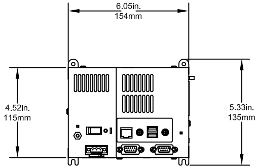
XP 00 Front View
