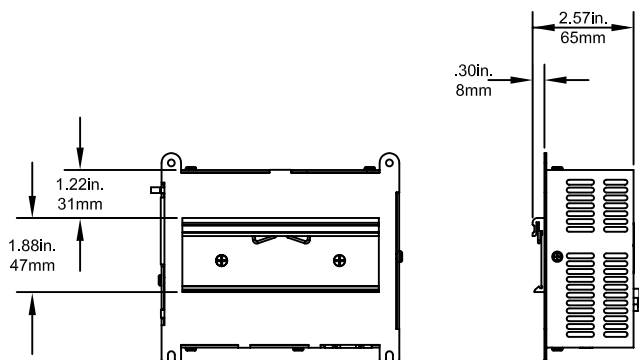
XP 00 with Din Rail Mount
