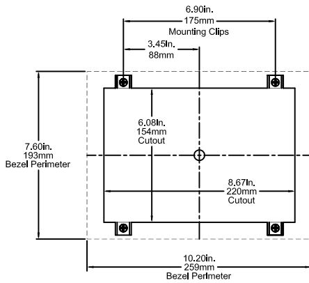
XP 8" Mounting
