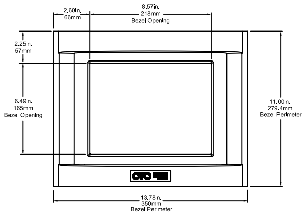
XP 10" Front View
