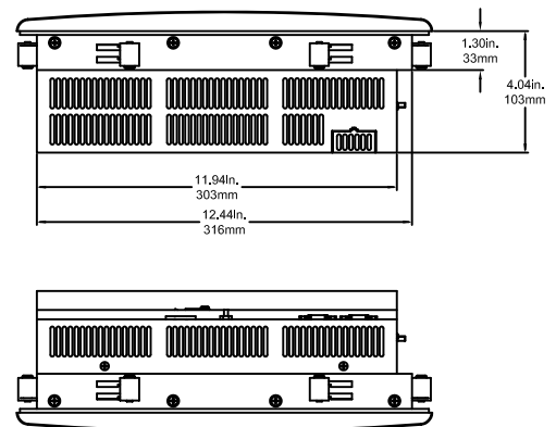
XP 10" Top and Bottom View
