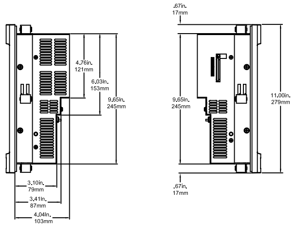
XP 10" Side Views
