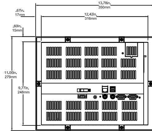
XP 10" Back View
